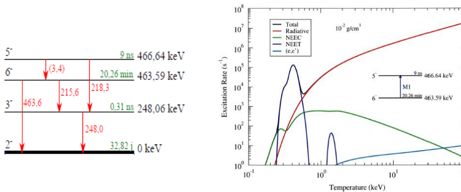
Figure 9 – Partial level scheme of ^{84}\text{Rb} and the rate for excitation of the 5^- state through different processes [55].
