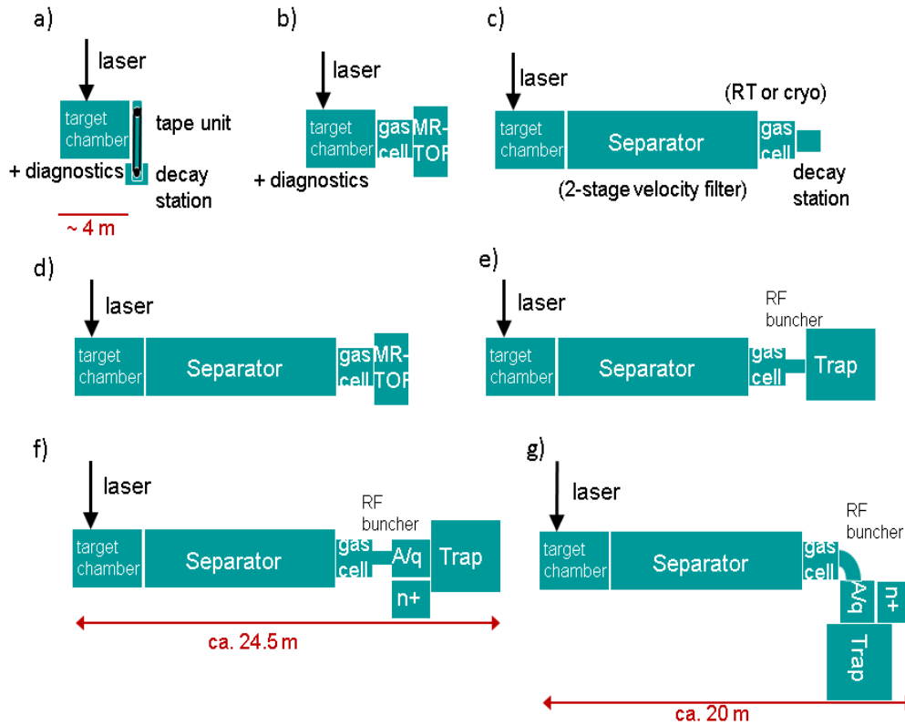
Figure 5 – Schematical view of the experimental arrangement for fission-fusion studies for different phases of the experimental development process. Measurements of fusion products will be performed primarily in two stages, first aiming at an identification of the produced isotopes via decay spectroscopy using a transport system (e.g. tape) directly behind the target chamber (a), or after thermalization in a buffer gas stopping cell and separation in a (multi-reflection) time-of-flight separator (MR-TOF) as developed by the Giessen group [41] (b) while later on a separator (e.g. 2-stage velocity filter) selects the ions of interest in order to prepare them (again after thermalization in the gas cell) either for selective spectroscopic studies (c) or for precision mass measurements either in the MR-TOF (d) or a Penning trap mass spectrometer (e), the latter potentially operated with highly-charged ions to increase the performance (f). In case of length problems of the setup to be integrated into the available floor space, also a (90 deg.) bent RFQ for extraction and bunching could be foreseen.
